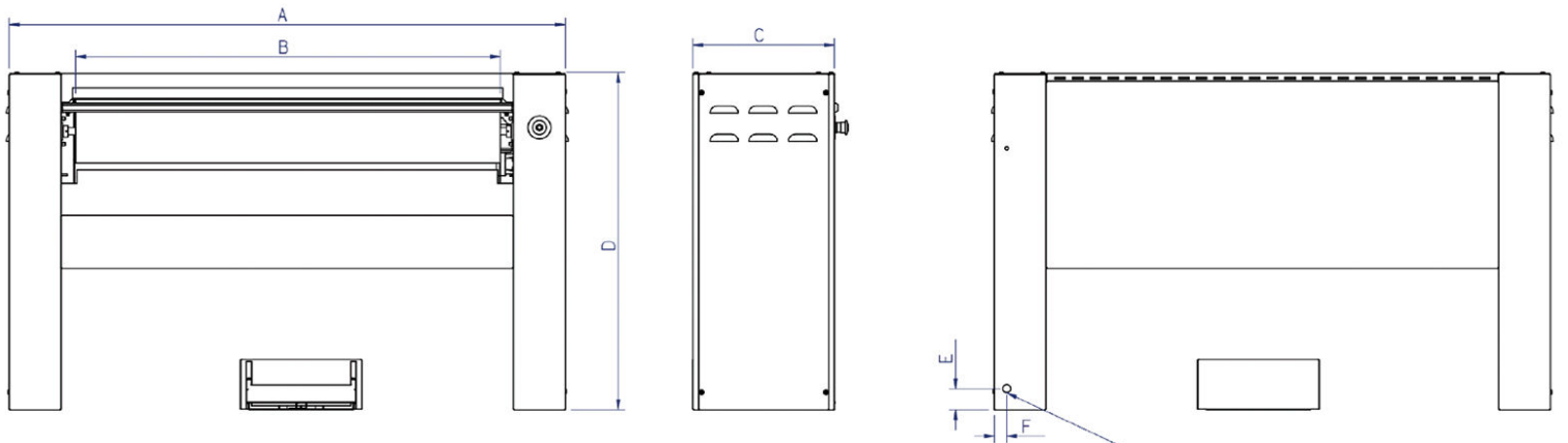
1. Electrical connection
