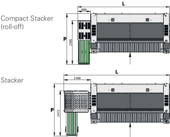
Compact Stacker
