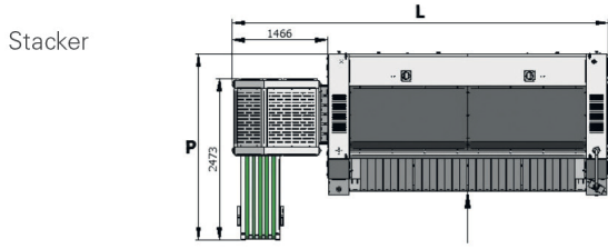
Compact Stacker
